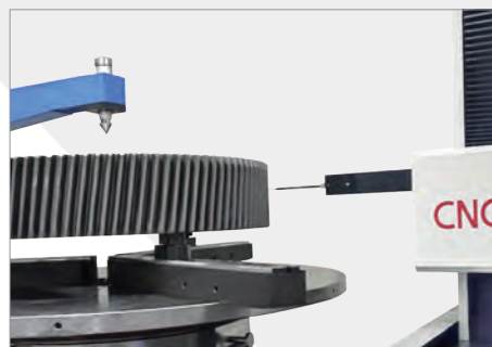
测量大型齿轮 Measure large gear
