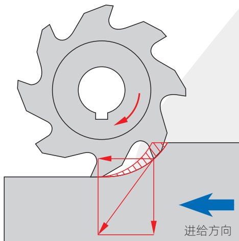
顺铣 Reverse Milling
