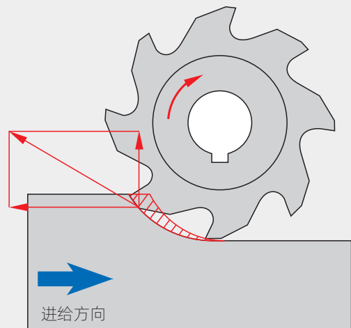
逆铣 Down Milling
